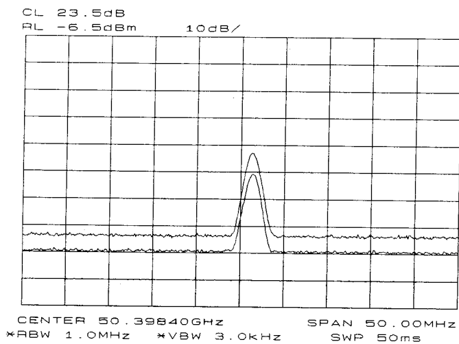
Figure 3-35. Response for Valid Signals
