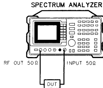
Figure 3-16. Transmission Measurement Test Setup
