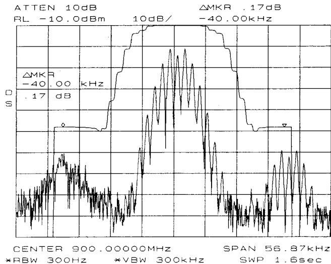
Figure 2-4. ACP Graph Display
