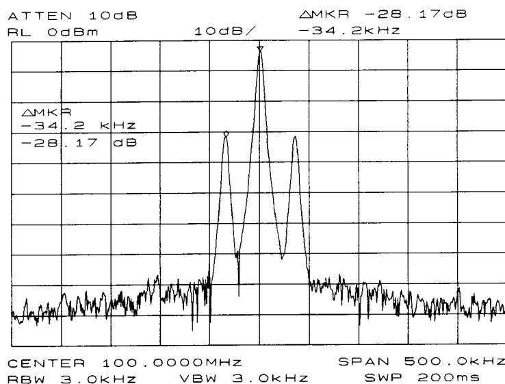
Figure H-1. An Amplitude-Modulated Signal
