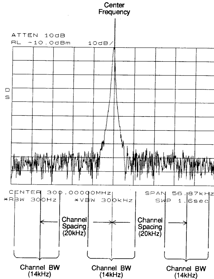
Figure 3-39. Adjacent Channel Power Parameters
