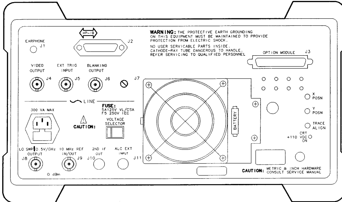
Figure 1-3. HP 8560A Rear Panel
