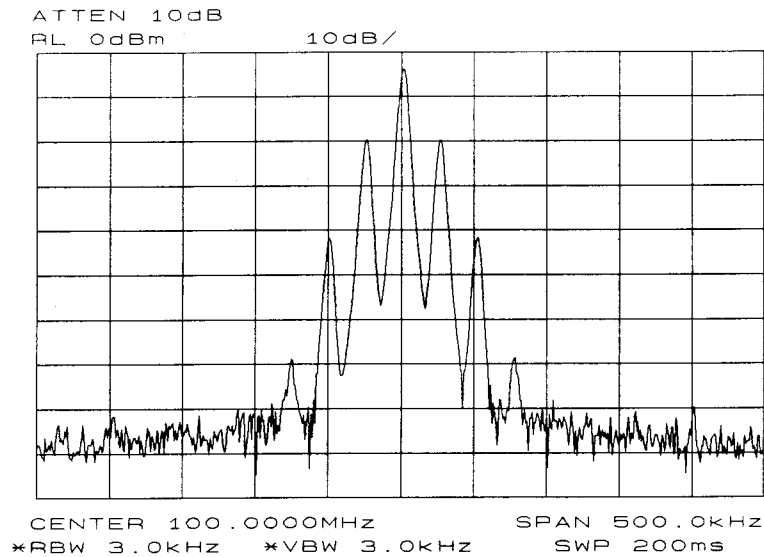
Figure H-3. A Frequency-Modulated Signal
