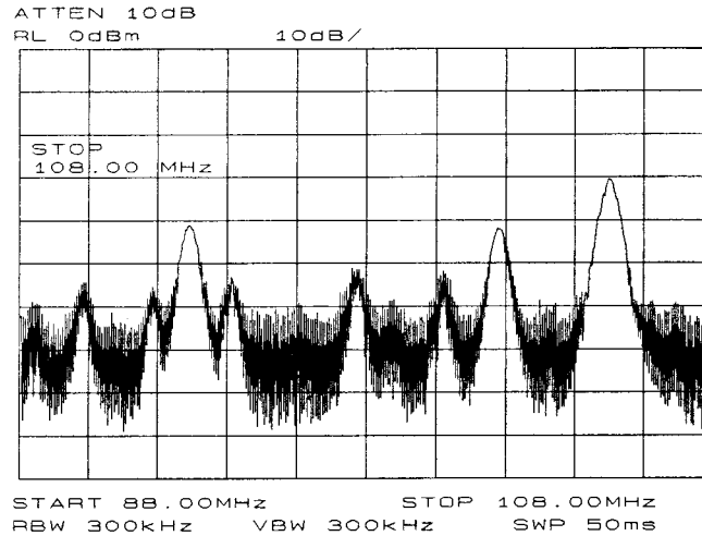
Figure 3-13. FM Band
