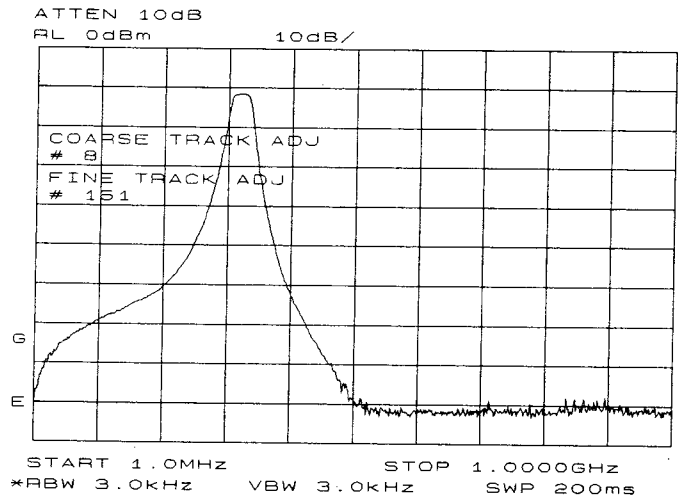
Figure 3-20. Manual tracking adjustment compensates for tracking error.
