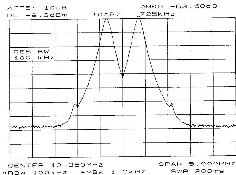
Figure G-4. 100 kHz Bandwidth Resolution
