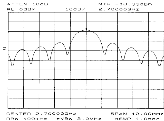
Figure I-3. Center Frequency at Center of Main Lobe
