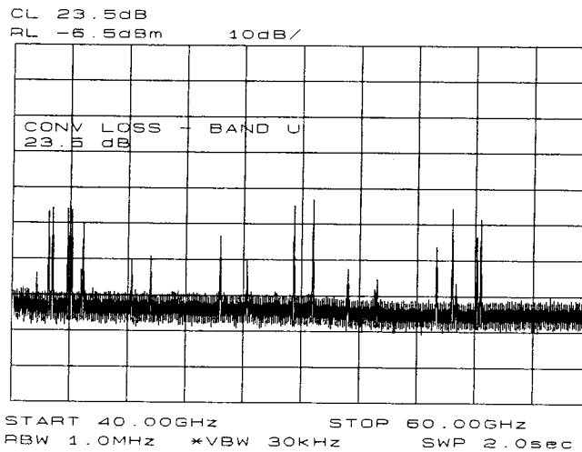
Figure 3-32. Store and correct for conversion loss.
