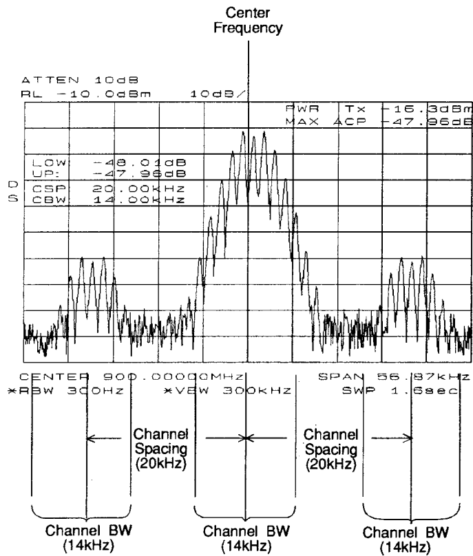
Figure 2-3. Channel Bandwidth Parameters
