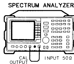
Figure 3-38. Adjacent Channel Power Measurement Test Setup
